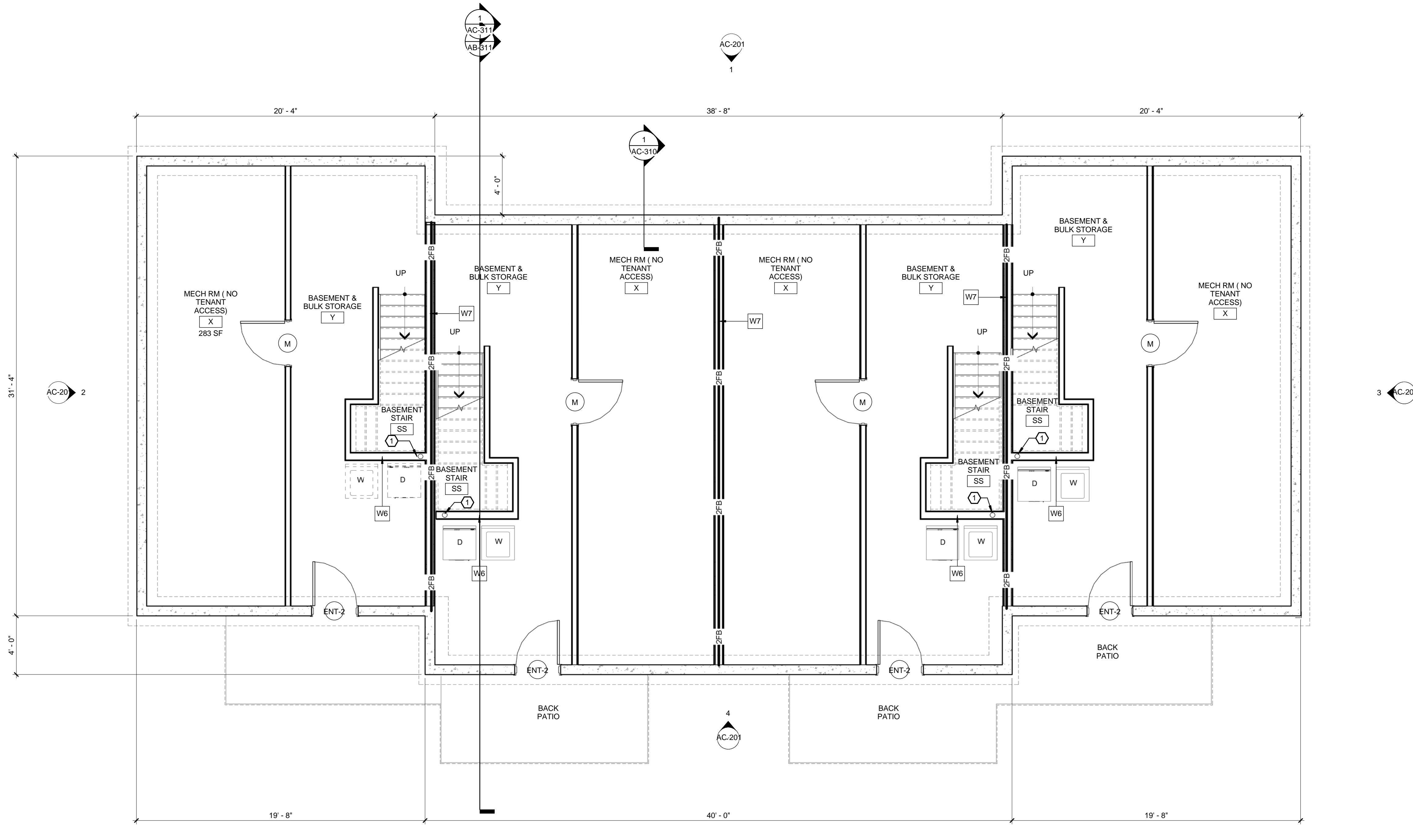
1 C-BASEMENT FLOOR PLAN 1/4" = 1'-0"
