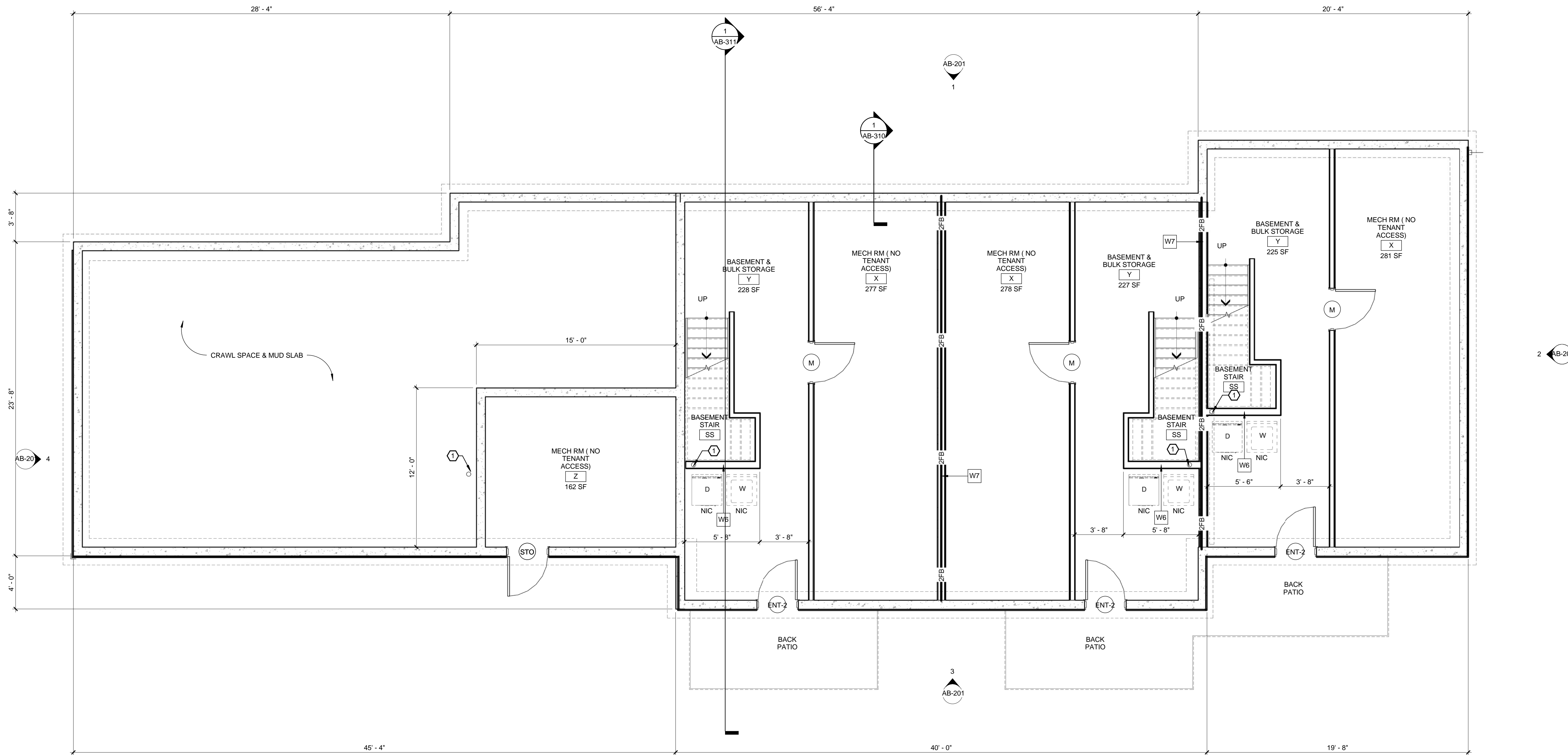
1 B- BASEMENT FLOOR PLAN 1/4" = 1'-0"
